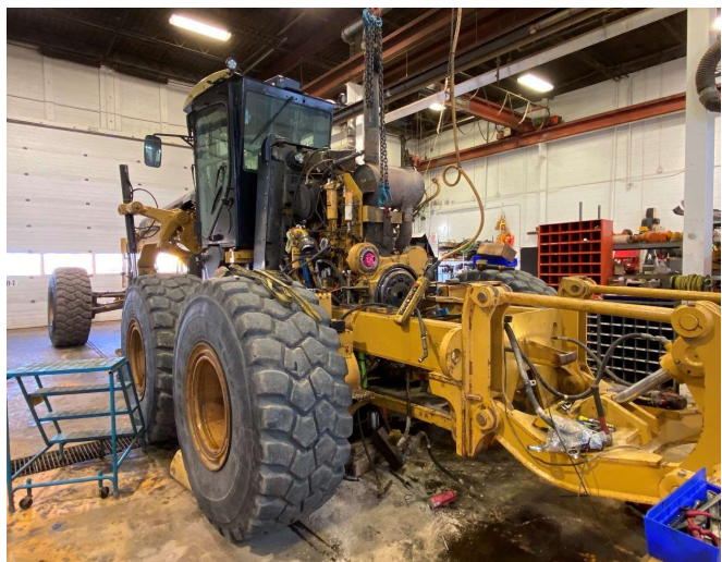
Right Side — Engine Bay (Transmission Removed)
