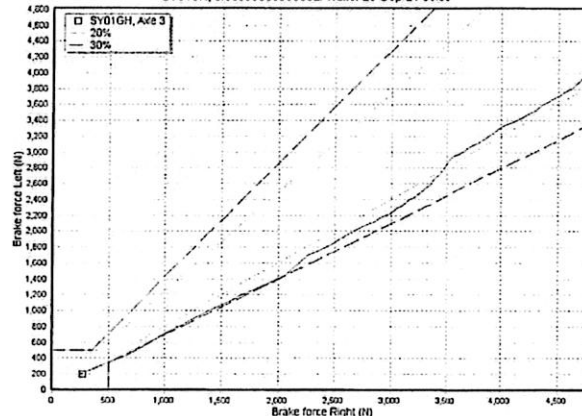
Brake Imbalance Chart Axle 3
