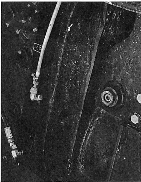
Dowel bolt broken.
