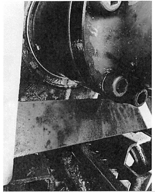
Watery gear oil leaking from the front seal.
