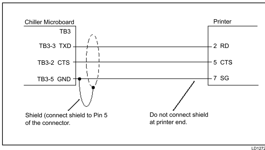
FIGURE 34 - PRINTER TO MICROBOARD ELECTRICAL CONNECTIONS
