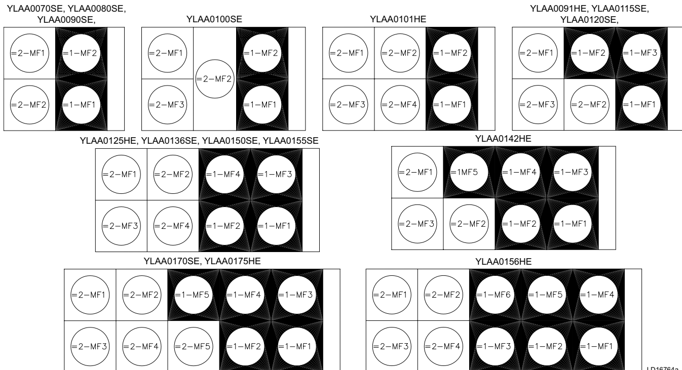
FIGURE 31 - CONDENSER FAN LOCATIONS
