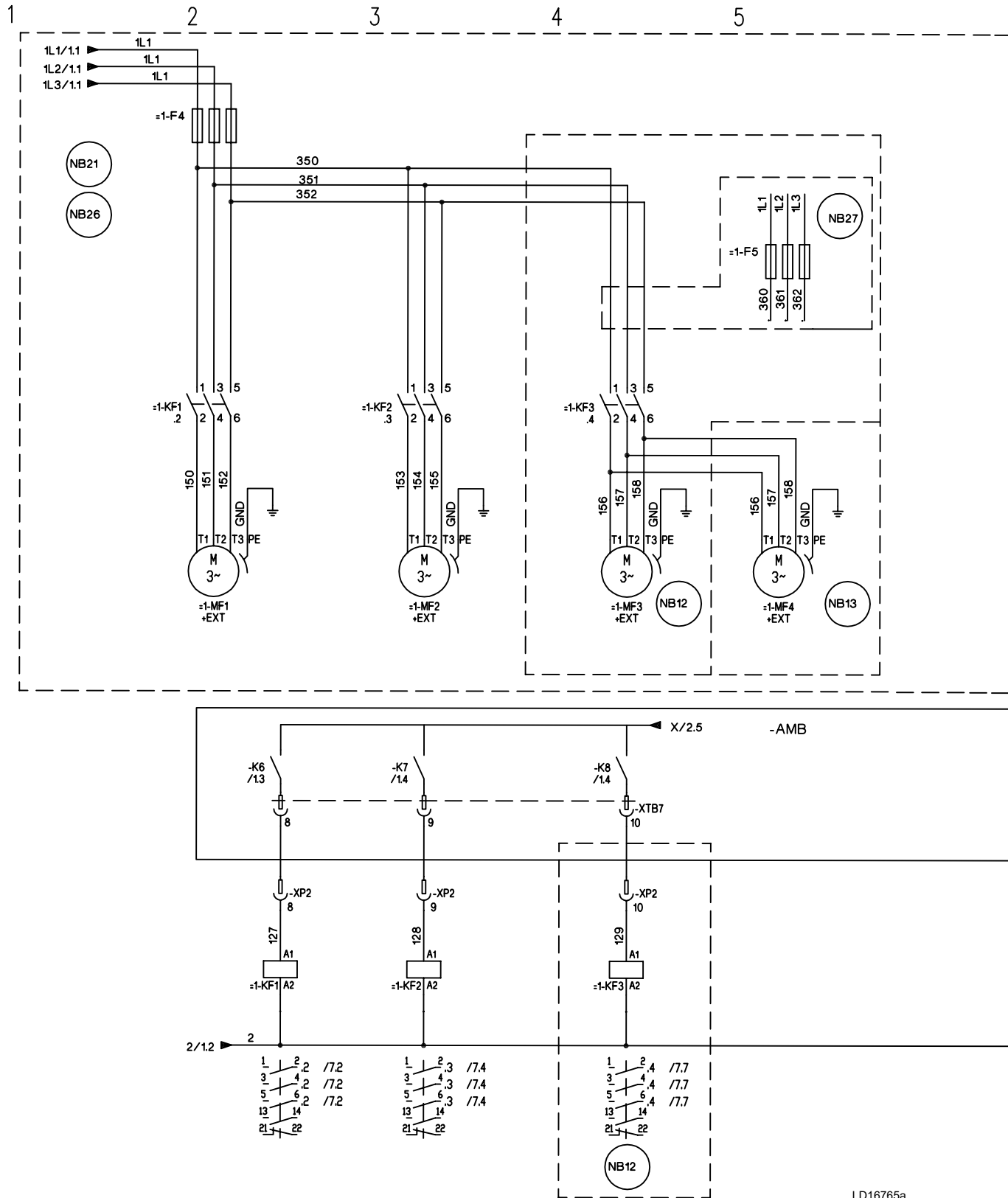
FIGURE 14 - FAN WIRING, STANDARD LOW SOUND OR ULTRA QUIET, YLAA0070 - YLAA0516
