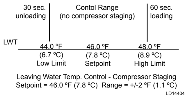
FIGURE 29 - LEAVING WATER TEMPERATURE CONTROL EXAMPLE
