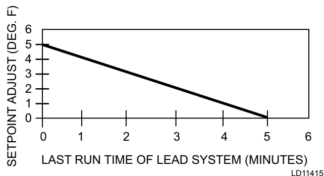
FIGURE 30 - SETPOINT ADJUST
