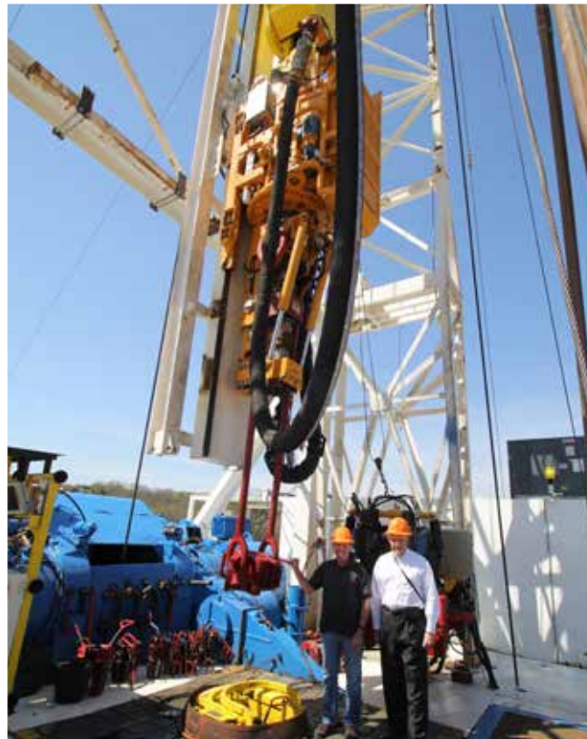
CanRig 275-T Top Drive
