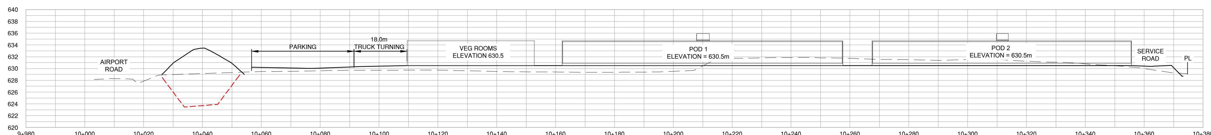
A EAST WEST SITE SECTION 1:750 1:375
