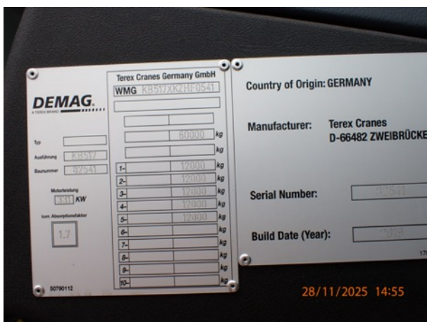
Photo 1: Serial plate
