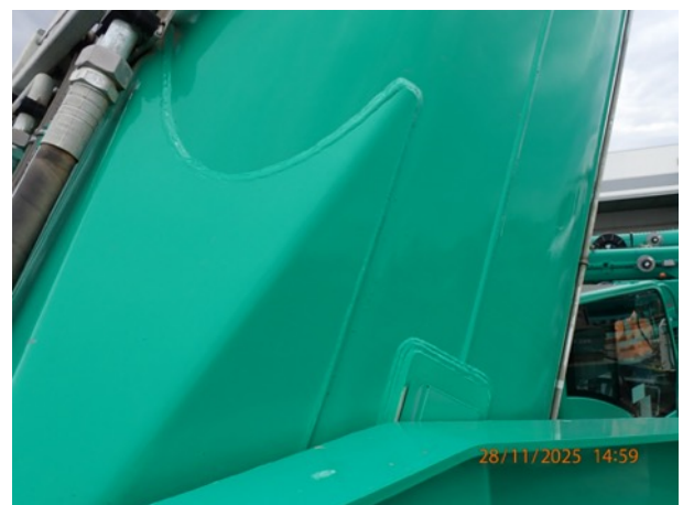
Photo 16: Boom welds
