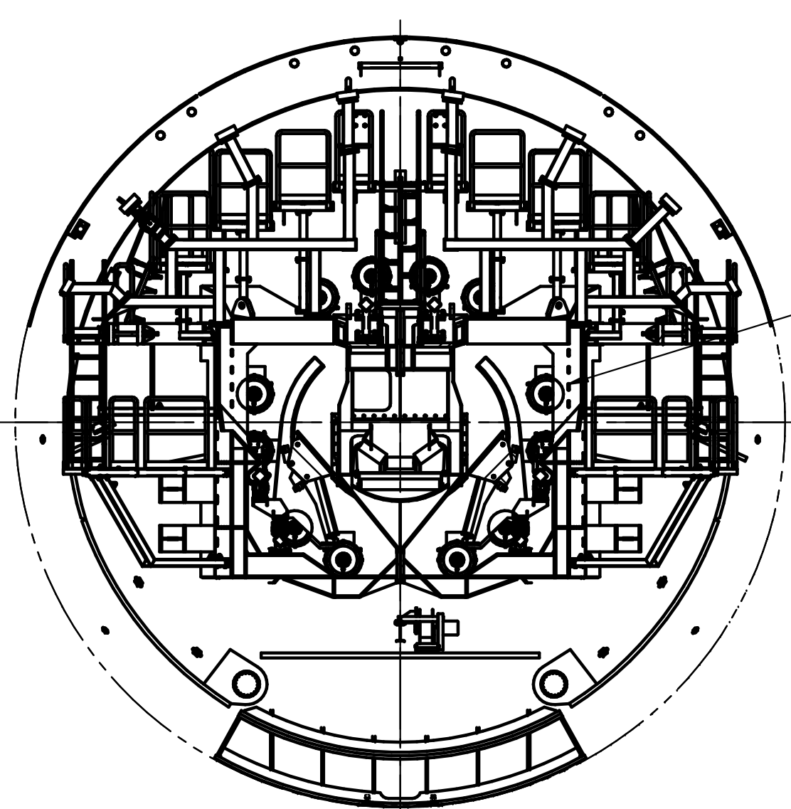
SECTION D-D (SHT 1) MESH ERECTOR
