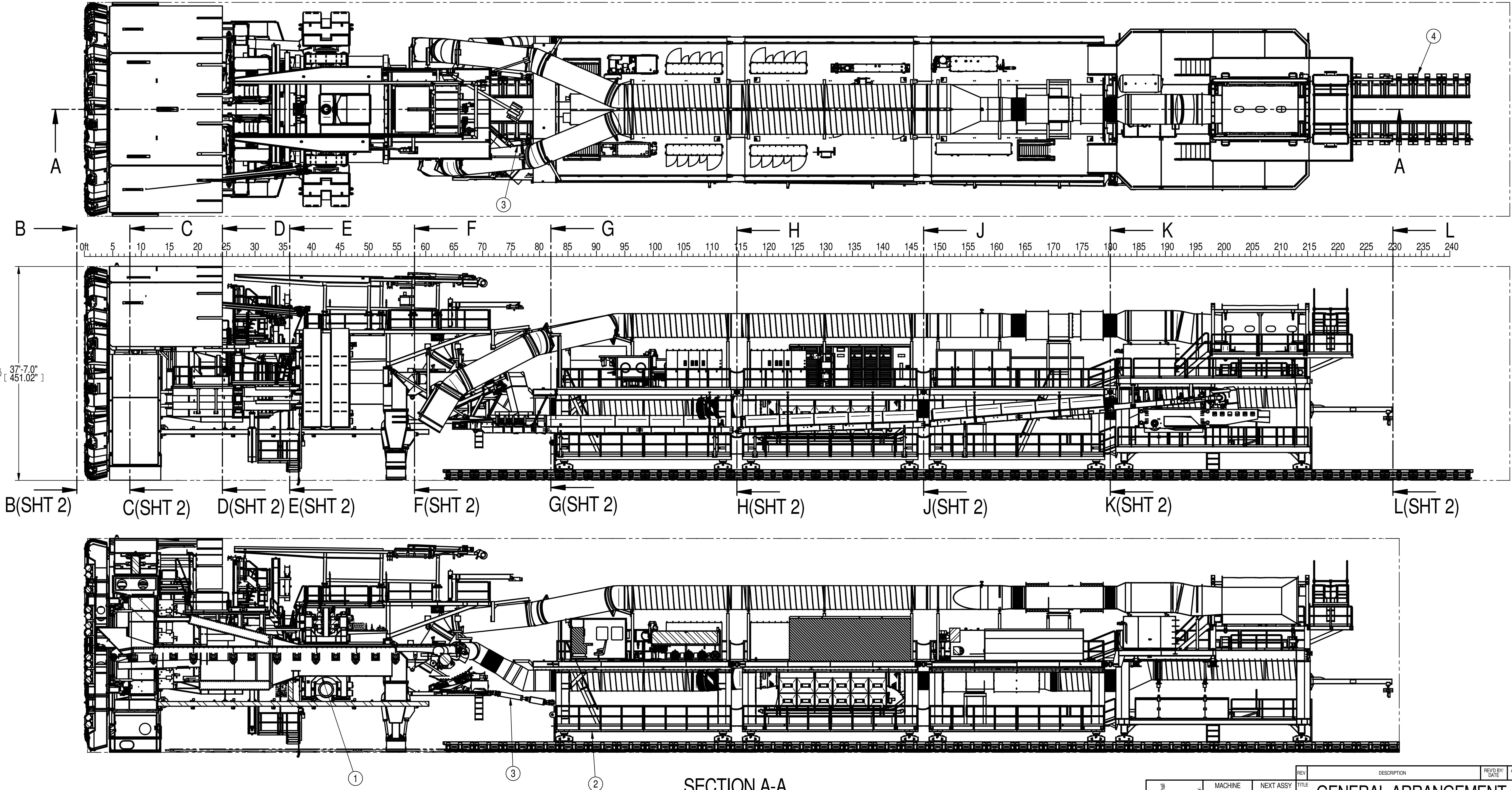
SECTION A-A TRC P/N 1133551 GENERAL ARRANGEMENT, TBM & BACKUP, 37'-7" ← FORWARD
