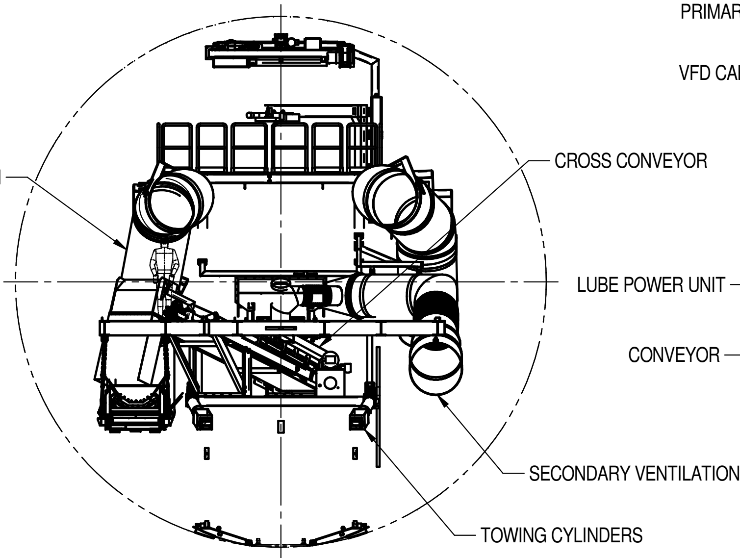
SECTION G-G (SHT 1) CROSS CONVEYOR & TOWING
