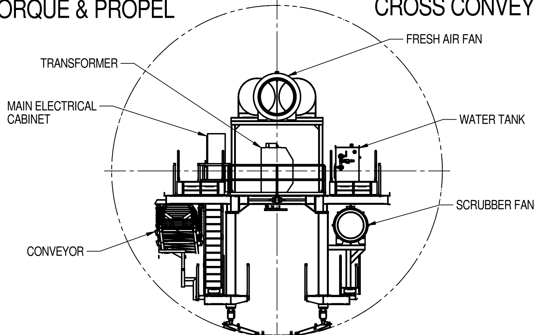
SECTION K-K (SHT 1) GANTRY 3
