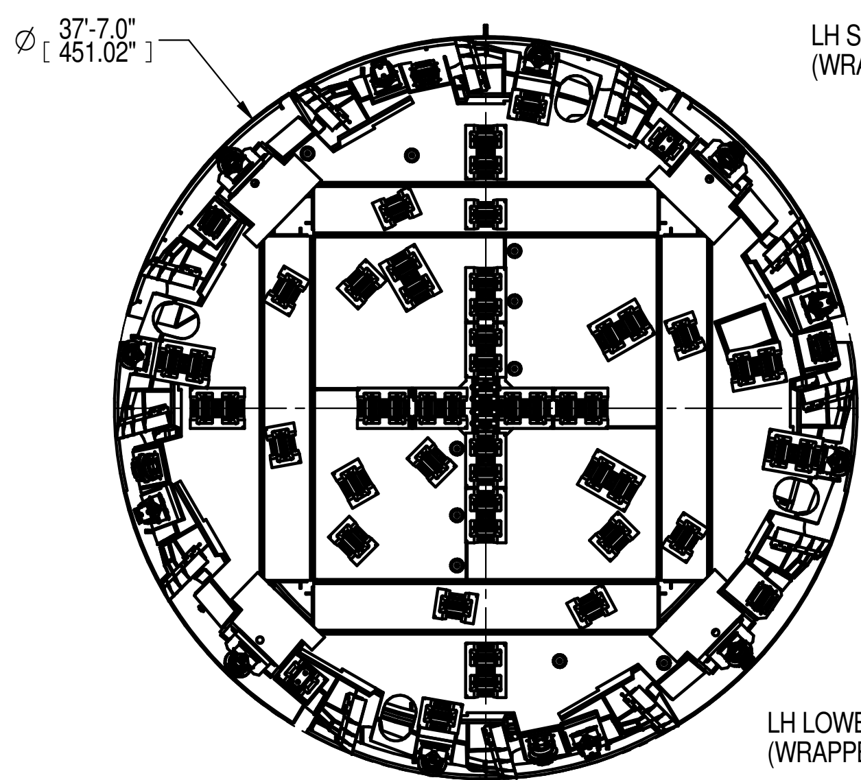
SECTION B-B (SHT 1) CUTTERHEAD
