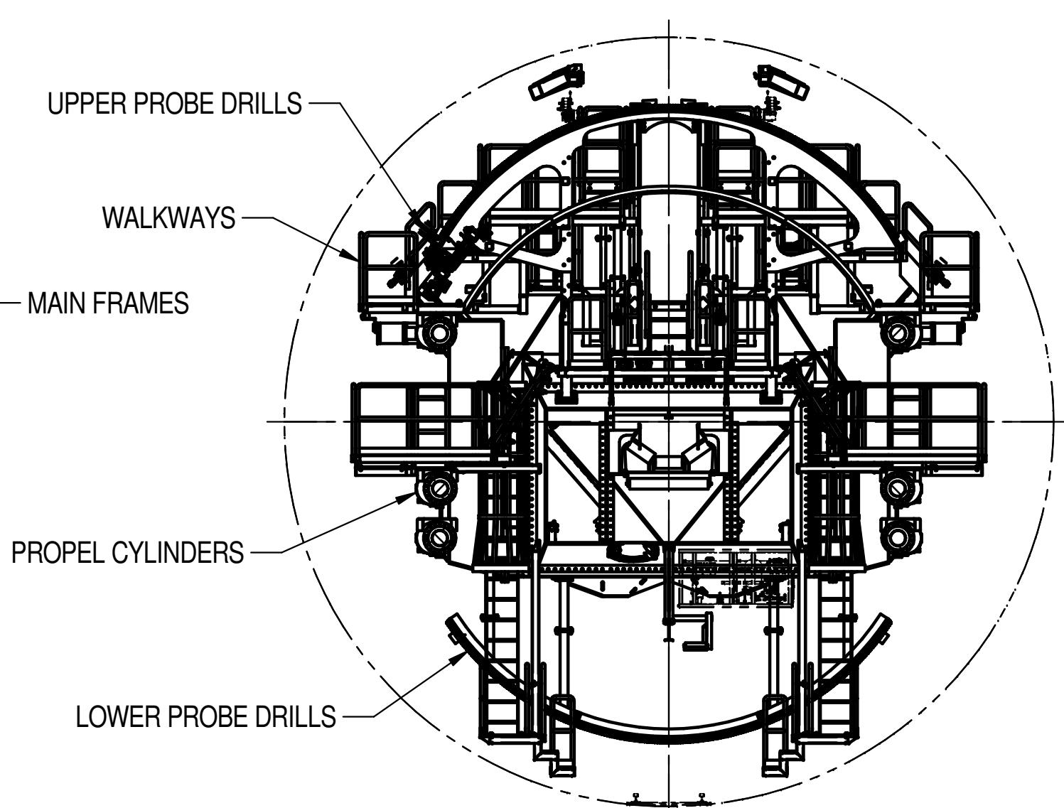
SECTION E-E (SHT 1) ROOF & PROBE DRILLS
