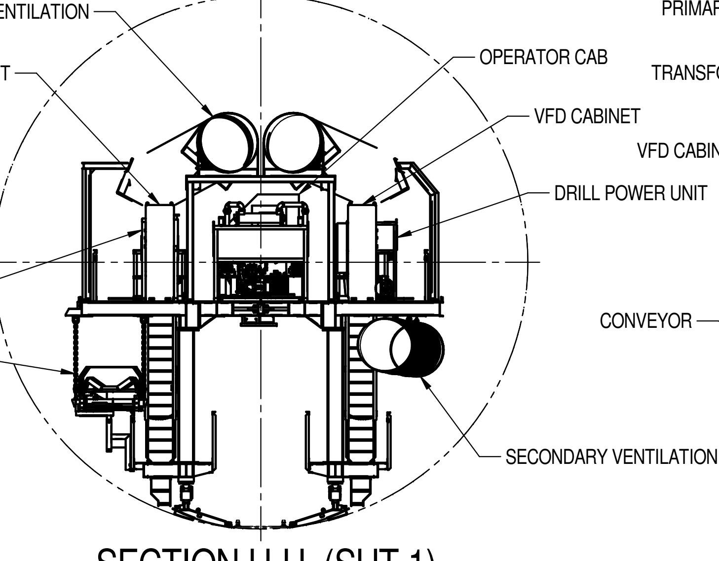
SECTION H-H (SHT 1) GANTRY 1
