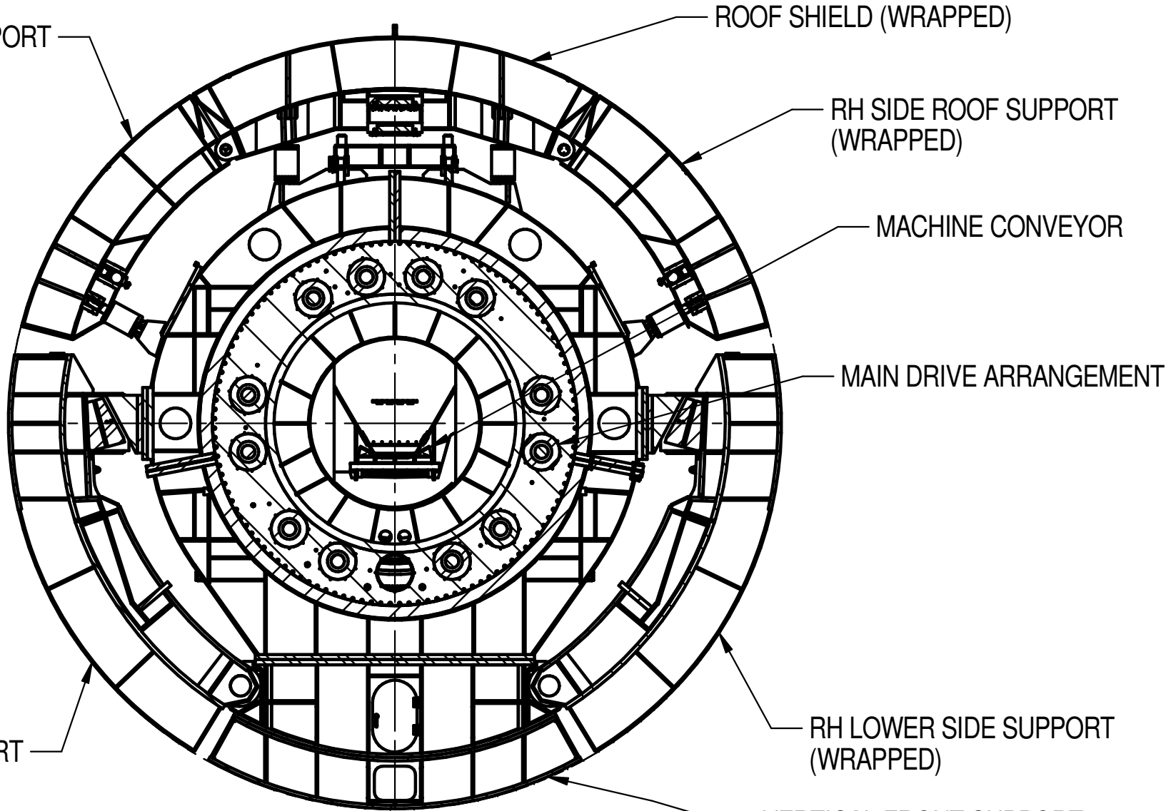
SECTION C-C (SHT 1) MAIN DRIVE
