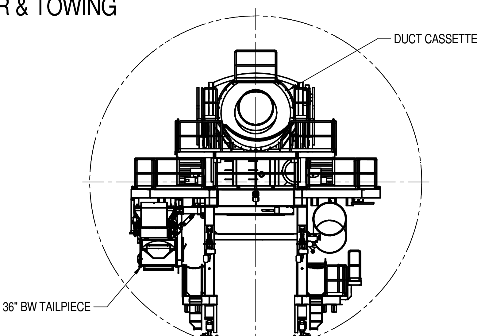
SECTION L-L (SHT 1) GANTRY 4
