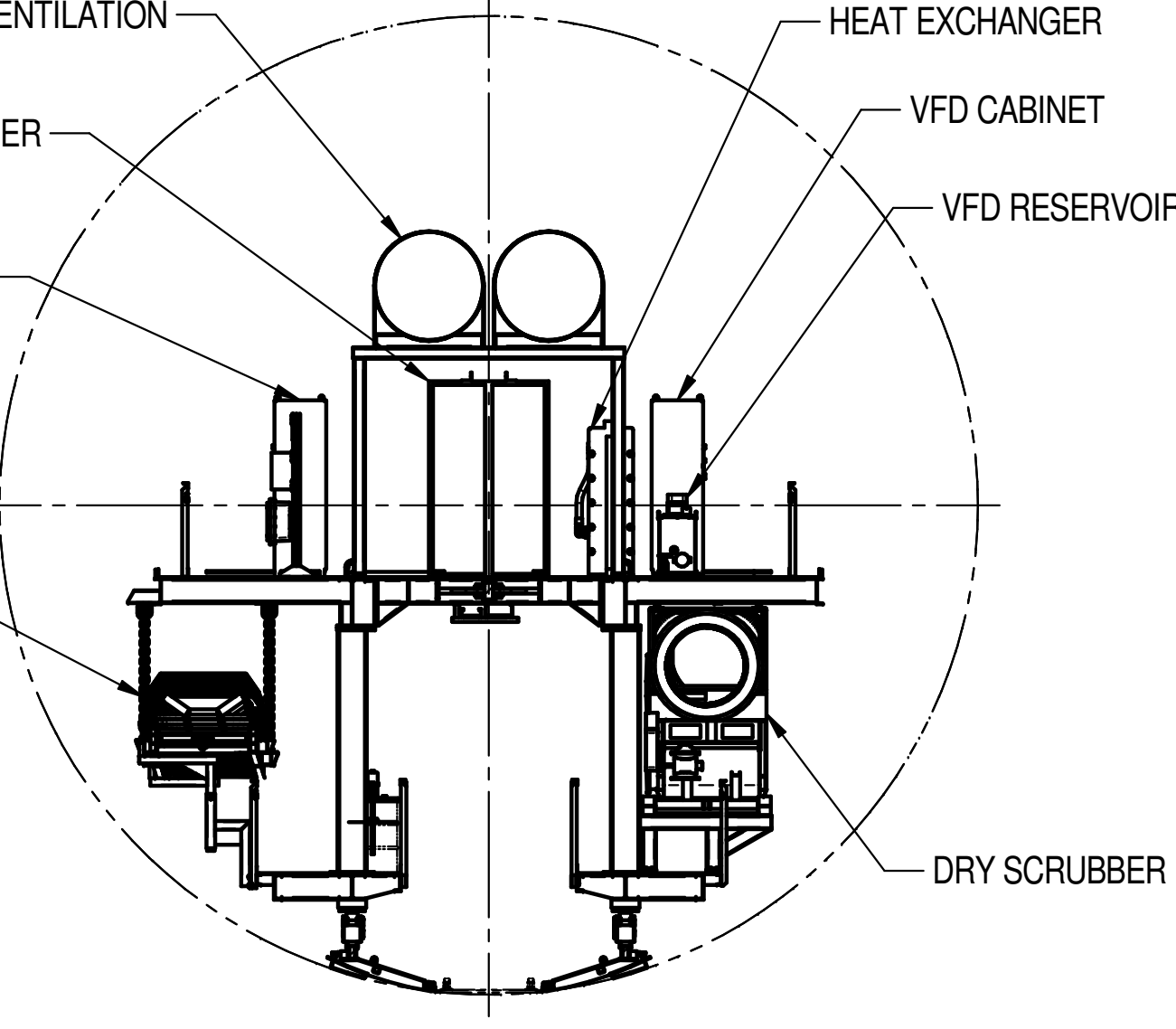
SECTION J-J (SHT 1) GANTRY 2
