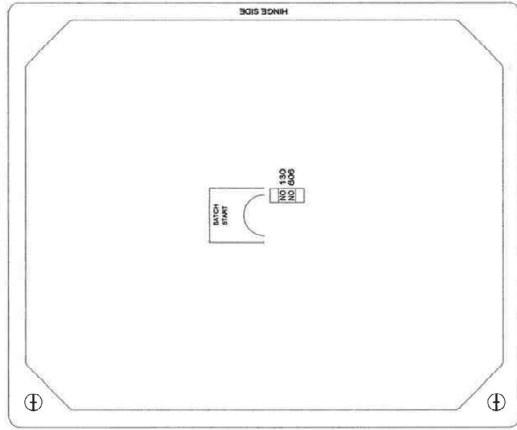
BACK OF DOOR LAYOUT AND FINISHING
