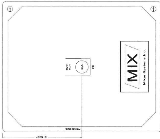
PAGE OF DOOR LAYOUT AND FINISHING
