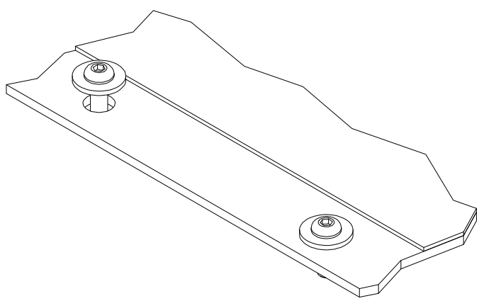
ALTERNATIVE DETAIL 'X' (SCALE:- 1 : 5) AS AN ALTERNATIVE TO SLOTS USE DIA 30 HOLES WITH OVERSIZE WASHERS (50 O/D x 17 I/D x 5 THK) & M16x60 LONG BUTTON HEAD BOLTS
